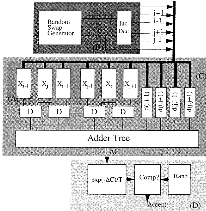
Fig 5. Architecture for solving the Travelling Salesman Problem
