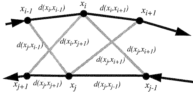
Fig 3. Effect of swapping two cities
