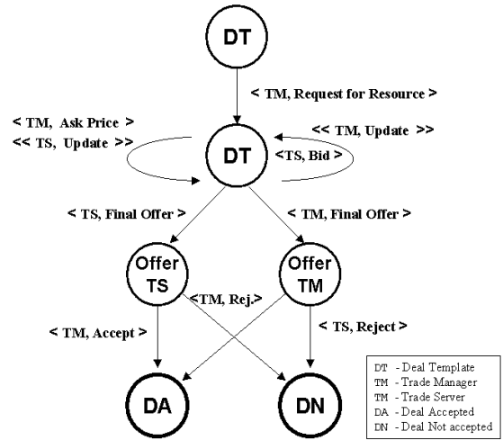
Figure 4: A finite state representation of resource trading negotiation (for market/bargain model).
