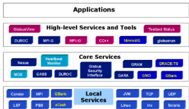
Figure 3: Economy Grid Components within Globus context.
