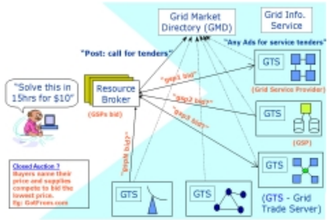
Figure 4: Tender/ContractNet model for resource trading.
