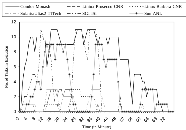
Figure 8: Resource Selection in Deadline and Budget based Scheduling for Time Optimization strategy.
