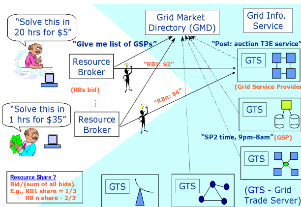
Figure 7: Market-based Proportional Resource Sharing.
