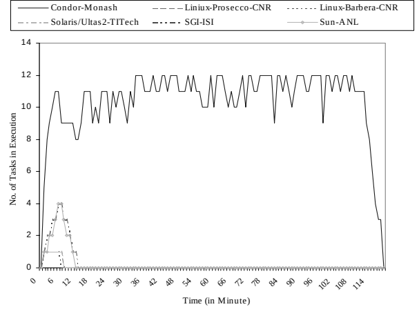
Figure 9: Resource Selection in Deadline and Budget based Scheduling for Cost Optimization strategy.
