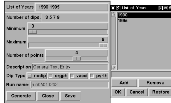
Figure 2: Sample user interface generated by template
