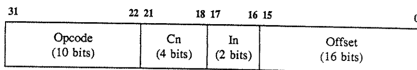
Figure 3 - A MONADS-PC instruction
