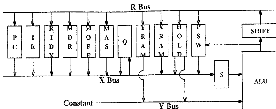
Figure 4 - the MONADS-PC bus structure
