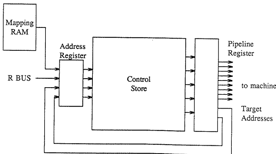
Figure 6 - the control unit
