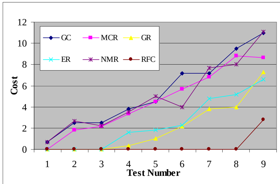
Graph 1 - Comparison of solution quality for different schemes.
