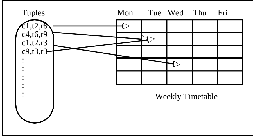
Figure 1 Mapping Tuples onto periods
