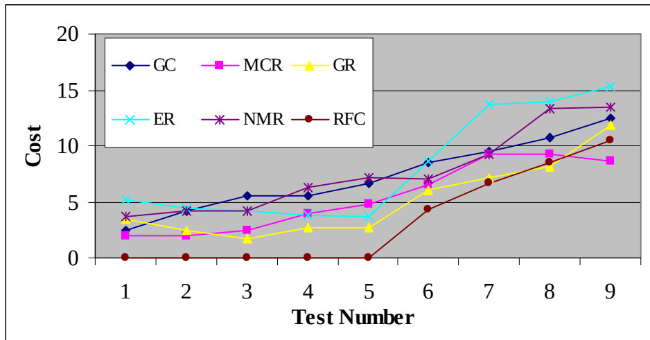
Graph 3 - Comparison of solution quality for same time
