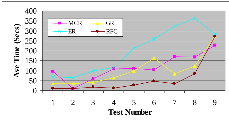
Graph 2 - Comparison of solution times for same quality
